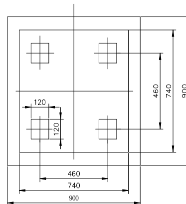
Foundation drawing
